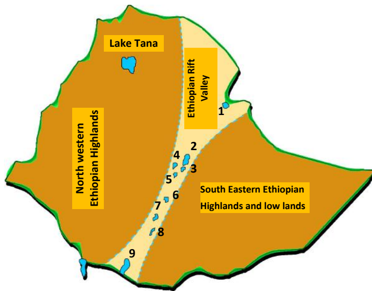
Fig. 1.12 The Ethiopian Rift Valley Lakes
